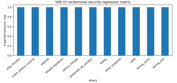
Fig. 4. Verified Execution Broker V2 reference stress test. Each condition uses 120 distinct randomized states/arguments; valid cases commit and all tested invalid/crash conditions fail closed. This figure is evidence for the isolated reference broker, not production integration.
